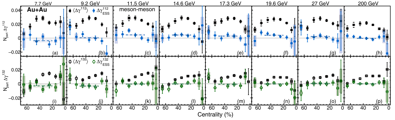
Fig. 4. (color online) Centrality dependence of (a–h) N_{\text{part}}\Delta\gamma^{112} and (i–p) N_{\text{part}}\Delta\gamma^{132} in Au+Au collisions at \sqrt{s_{\text{NN}}} = 7.7\text{--}200 GeV. Both the ensemble averages (squares) and the ESS results (circles) are presented. The error bars, shaded boxes, and brackets represent statistical uncertainties, measurement systematics, and uncertainties associated with N_{\text{part}} , respectively. The dashed lines represent constant fits over the 20%–50% centrality range. The shaded bands denote the fit uncertainties.
