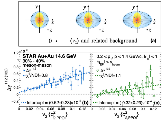
Fig. 3. (color online) Upper: (a) illustration of various particle emission patterns (outer regions spanned by arrows) for different events with the same initial geometry (inner elliptic regions). Image reproduced and modified from Ref. [40]. Lower: (b) \Delta\gamma^{112} and (c) \Delta\gamma^{132} as a function of v_2 with events categorized by q_{2,\text{PPOI}}^2 in the 30%–40% centrality range of Au+Au collisions at \sqrt{s_{NN}} = 14.6 GeV. POI are charged hadrons, excluding (anti)protons. The ESS technique extrapolates an observable to isotropic emission, characterized by zero elliptic flow ( v_2 ). The error bars are statistical only. Linear fits (dashed lines) are used to extract the y-intercepts, with \chi^2/\text{NDF} close to unity.
