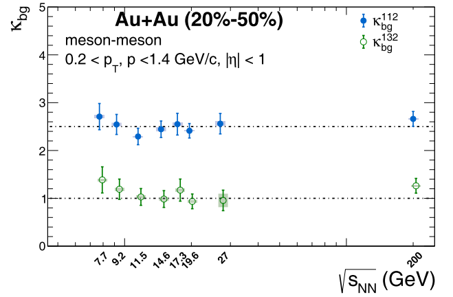
Fig. 6. (color online) Beam-energy dependence of \kappa_{\text{bg}}^{112} (full circles) and \kappa_{\text{bg}}^{132} (open circles) integrated over the 20%–50% centrality range in Au+Au collisions. Error bars represent statistical uncertainties, and shaded boxes denote systematic uncertainties. The dashed lines at 2.5 and 1 are drawn to guide the eye.
