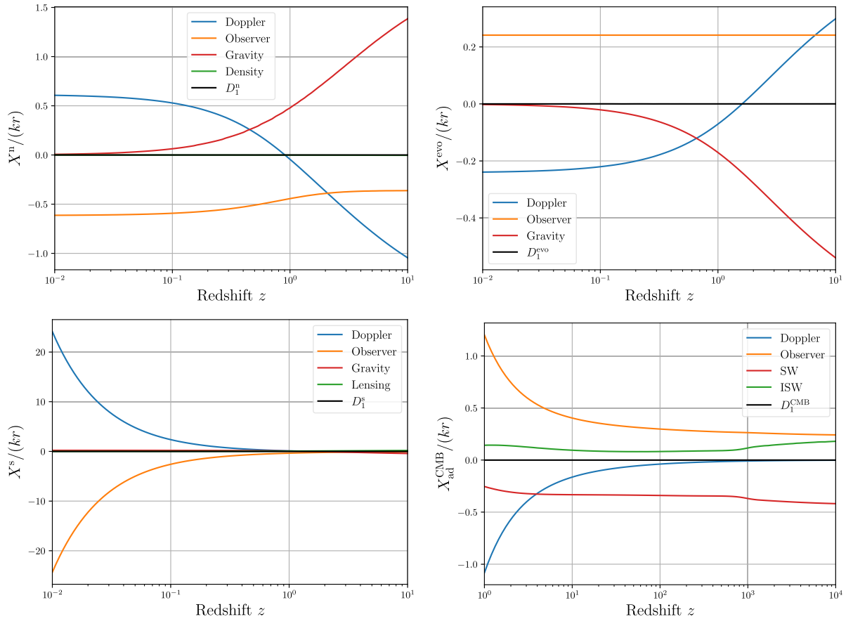
Fig. 1. (color online) Contributions to the number-count dipole and the CMB dipole for a single Fourier mode under adiabatic initial conditions. The first three panels show the contributions to D_1^n [top-left], D_1^{\text{evo}} [top-right], and D_1^s [bottom-left], as defined in Eq. (13). The last panel shows the contributions to D_1^{\text{CMB}} [bottom-right] from the Sachs-Wolfe effect, the Doppler effect, the integrated Sachs-Wolfe effect, and the observer term. Notably, an exact cancellation occurs, yielding D_1 = 0 (black) to leading order in both the CMB and number-count dipoles for adiabatic initial conditions.
