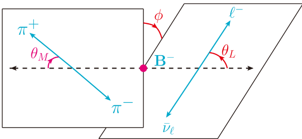
Fig. 2. (color online) The angular variables (\theta_M, \theta_L, \phi) in the four-body B^- \rightarrow \pi^+ \pi^- \ell^- \bar{\nu}_\ell decay.
