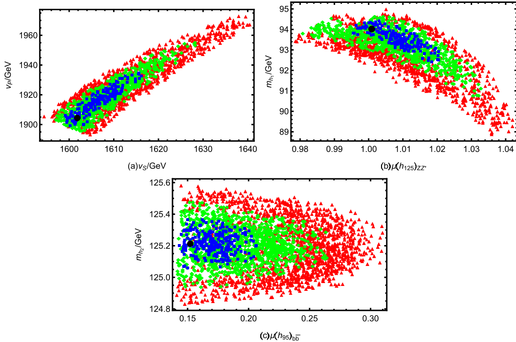
Fig. 4. (color online) The symbols denote the \chi^2 confidence regions: • marks the best-fit point ( \chi^2_{\min} = 4.39 ), ■ the 1\sigma region ( \chi^2 \leq 6.69 ), ♦ the 1-2\sigma region ( 6.69 < \chi^2 \leq 10.57 ), and ▲ the 2-3\sigma region ( 10.57 < \chi^2 \leq 16.22 ).
