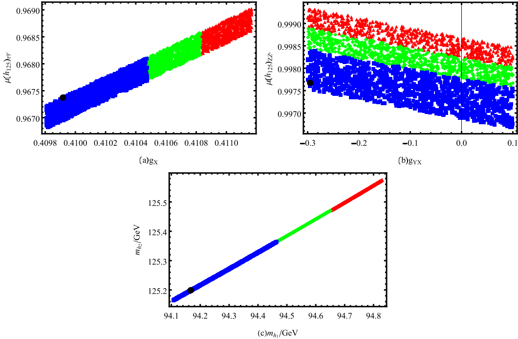
Fig. 5. (color online) The symbols denote the \chi^2 confidence regions: \bullet marks the best-fit point ( \chi^2_{\min} = 4.41 ); \blacksquare the 1\sigma region ( \chi^2 \leq 6.71 ); \blacklozenge the 1-2\sigma region ( 6.71 < \chi^2 \leq 10.59 ); and \blacktriangle the 2-3\sigma region ( 10.59 < \chi^2 \leq 16.24 ).
