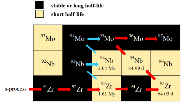
Fig. 1. (color online) S-process path in the region of ^{94}\text{Mo} .
