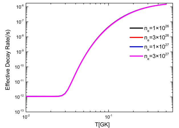
Fig. 3. (color online) Effective decay rate of ^{94}\text{Nb} as a function of temperature and electron number density.
