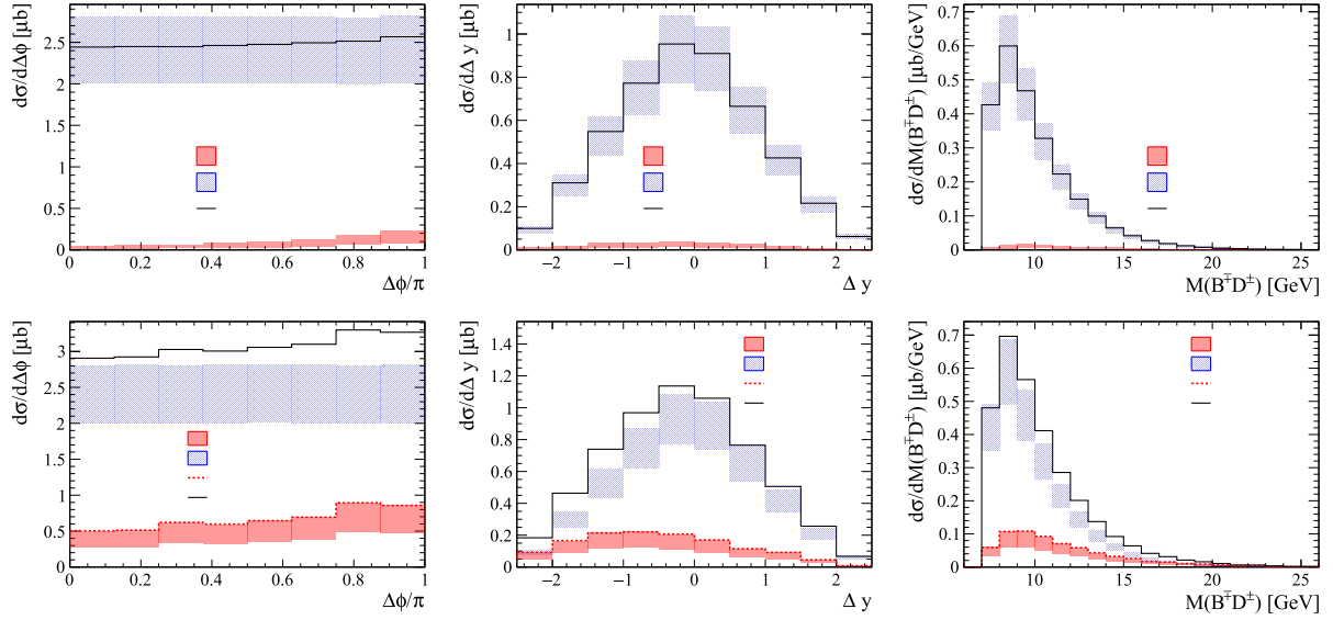
Fig. 2. (color online) Differential cross sections for associated B^+ D^+ production via SPS and DPS. Left: \Delta\phi distribution; middle: \Delta y distribution; right: invariant-mass M(B^+ D^+) distribution, shown for \sigma_{\text{eff}} = 15 mb. The upper (lower) panels show the SPS prediction at NLO in the 3FNS (LO in the 4FNS). The SPS contribution is displayed as a red shaded band, with uncertainties dominated by renormalization- and factorization-scale variations, while the DPS contribution is displayed as a blue hatched band. In the upper panels, the black solid line denotes the combined SPS+DPS central prediction, which defines the baseline background scenario. In the lower panels, the red dashed line indicates the maximal SPS contribution, taken from the upper bound of the LO 4FNS prediction, while the black solid line shows the corresponding SPS (max)+DPS prediction, which defines the conservative maximal background scenario.
