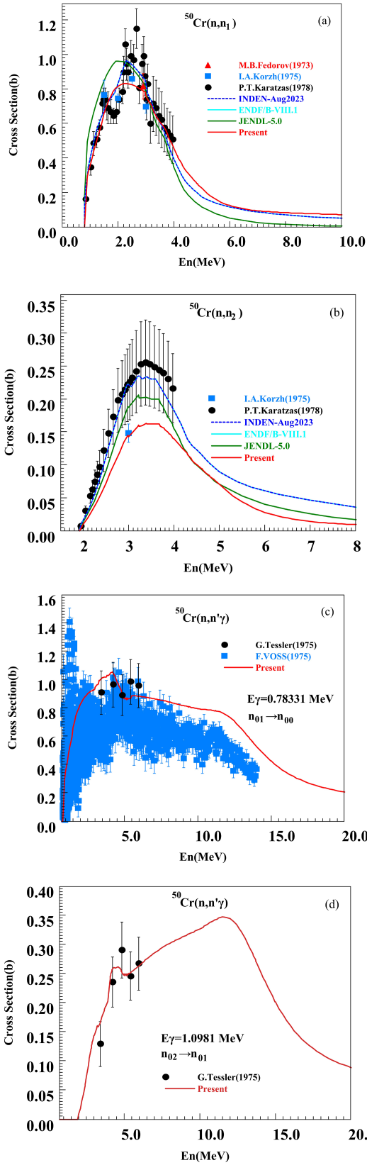
Fig. 16. (color online) Comparison of discrete level inelastic cross sections and inelastic scattering gamma production cross sections for ^{50}\text{Cr} between evaluated data (red curve) and experimental data (symbols).
