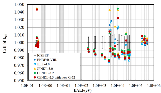
Fig. 37. (color online) Computed-to-experimental (C/E) ratios for Criticality Benchmark Validation of ^{52}\text{Cr}
