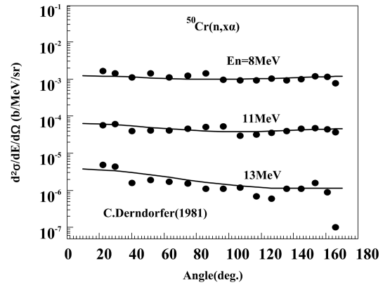
Fig. 34. Comparisons of double differential cross sections for alpha particle emission at incident energy of 8.0, 11.0, and 13.0 MeV between the evaluated data (solid curves) and experimental data reported by Derndorfer (1981) (symbols). In each panel, the topmost curve for 8.0 MeV follows the true reported values in the literature, and the other results from 11.0 MeV to 13.0 MeV are multiplied by factors of 0.1, 0.01, etc., respectively.
