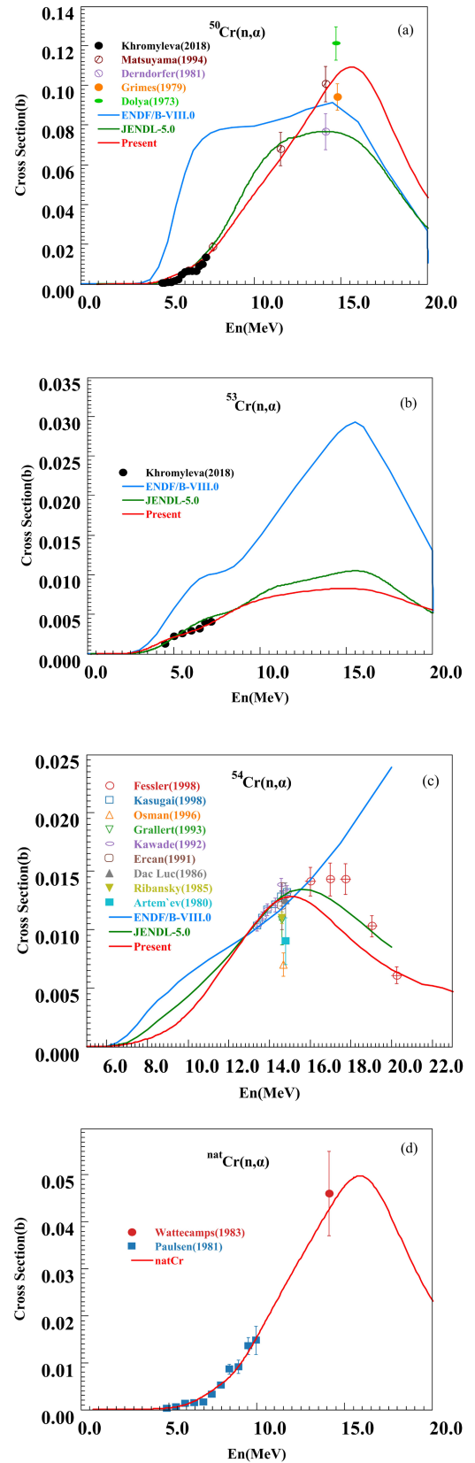
Fig. 20. (color online) Comparison of ^{50,53,54,\text{nat}}\text{Cr}(n,\alpha) cross sections between evaluated data (red curve) and experimental data (symbols).
