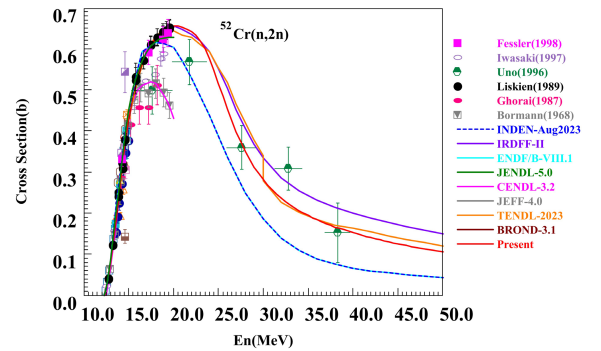
Fig. 4. (color online) Comparison of ^{52}\text{Cr}(n, 2n) cross sections between evaluated data (red curve) and experimental data (symbols).
