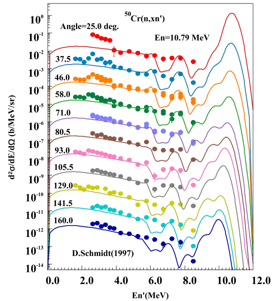
Fig. 29. (color online) Comparisons of ^{50}\text{Cr}(n, xn) double-differential cross sections at different angles for an incident energy of 10.79 MeV between the evaluated data (solid curves) and experimental data (symbols). The topmost curve for 25.0 degrees follows the true reported values in the literature, and the other results from 37.5 to 160.0 degrees are multiplied by factors of 0.1, 0.01, etc., respectively.
