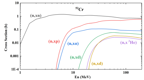
Fig. 26. (color online) Production cross sections of six fundamental particles ( n , p , d , t , ^3\text{He} , and \alpha ) below 200 MeV.
