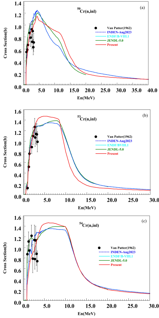
Fig. 14. (color online) Comparison of ^{50,53,54}\text{Cr}(n, \text{inel}) cross sections between evaluated data (red curve) and experimental data (symbols).
