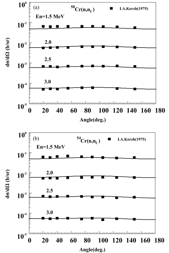
Fig. 10. Comparisons of inelastic scattering angular distributions for ^{50,54}\text{Cr}(n,n_1) between evaluated data (solid lines) and experimental data reported by Korzh et al. (1975) (symbols). The energy region covers from 1.5 MeV to 3.0 MeV. In each panel, the topmost curve for 1.5 MeV follows the true reported values in literature, and the other results from 1.5 MeV to 3.0 MeV are multiplied by factors of 0.1, 0.01, etc., respectively.
