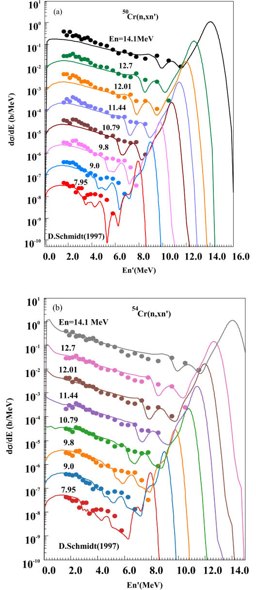
Fig. 36. (color online) Comparison of the neutron emission energy spectra for ^{50,54}\text{Cr} between the evaluated data (solid curves) and the experimental data reported by D. Schmidt (1997) (symbols). In each panel, the topmost curve for 14.1 MeV follows the true reported values in the literature, and the other results from 12.7 MeV to 7.95 MeV are multiplied by factors of 0.1, 0.01, etc., respectively.
