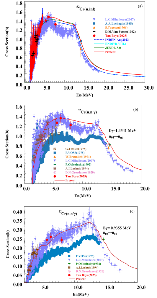
Fig. 15. (color online) Comparison of discrete level inelastic cross sections and inelastic scattering gamma production cross sections for ^{52}\text{Cr} between evaluated data (red curve) and experimental data (symbols).
