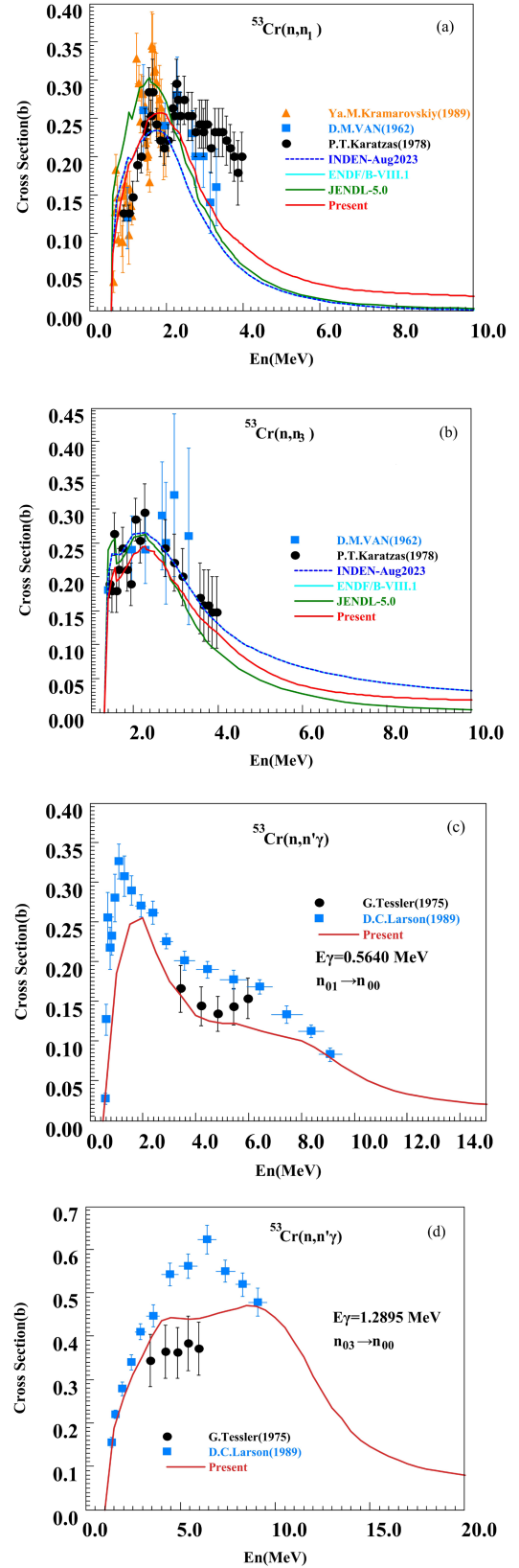
Fig. 17. (color online) Comparison of discrete level inelastic cross sections and inelastic scattering gamma production cross sections for ^{53}\text{Cr} between evaluated data (red curve) and experimental data (symbols).
