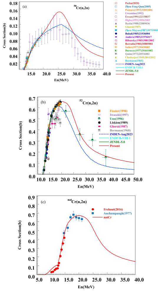
Fig. 21. (color online) Comparison of ^{50,52,\text{nat}}\text{Cr}(n,2n) cross sections between evaluated data (red curve) and experimental data (symbols).
