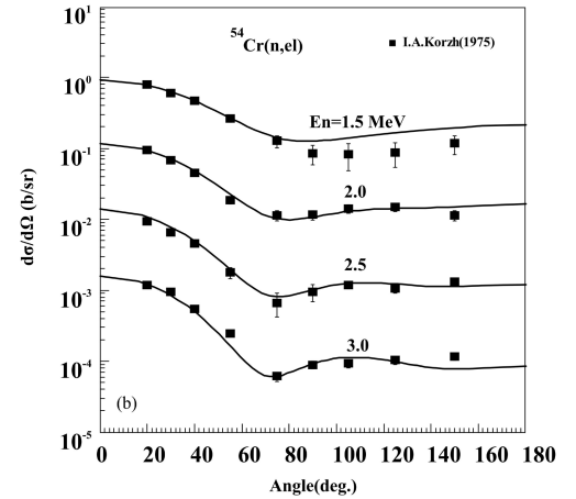
Fig. 8. Comparisons of elastic scattering angular distributions for ^{50,54}\text{Cr}(n,\text{el}) between evaluated data (solid lines) and experimental data reported by Korzh et al. (1975) (symbols). The energy region covers 1.5 MeV to 3.0 MeV. In each panel, the topmost curve for 1.5 MeV follows the true reported values in literature, and the other results from 1.5 MeV to 3.0 MeV are multiplied by factors of 0.1, 0.01, etc., respectively.
