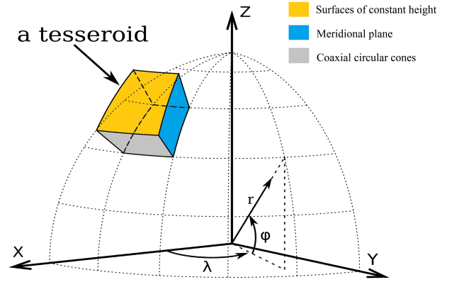
Fig. 1. (color online) Tesseroid Grid Schematic Diagram, Adapted from Uieda, 2015 [16].
