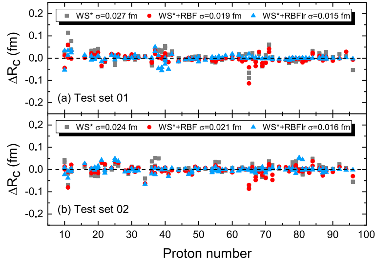
Fig. 4. (color online) Trend of the deviations between the theoretical and experimental charge radii of test sets 01 and 02 as a function of proton number. (a) The squares, dots, and triangles respectively represent the prediction results of the WS* radius formula and its combination with the RBF and RBFIr approaches for test set 01. (b) Same as (a) but for test set 02.
