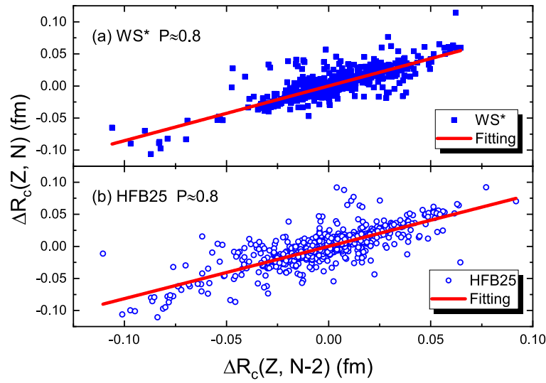
Fig. 1. (color online) Relationship between \Delta R_c(Z, N) and \Delta R_c(Z, N-2) . The squares and circles denote the results of the WS* radius formula and HFB25 model, respectively.
