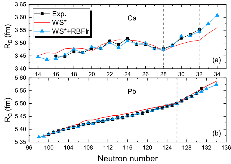
Fig. 5. (color online) Trend of charge radii of the Ca and Pb isotope chains with neutron number. Squares represent the experimental values, and vertical lines represent error bars. The solid lines and triangles represent the prediction results of the WS* radius formula and its combination with the RBF approach, respectively.
