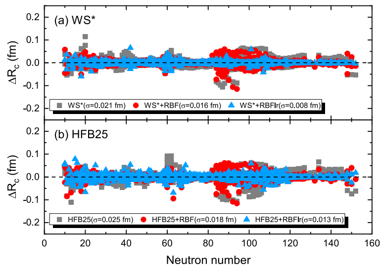
Fig. 2. (color online) Trend of the deviations between the theoretical and experimental charge radii of 855 neutron-rich nuclei as a function of the neutron number. (a) The squares, dots, and triangles respectively represent the prediction results of the WS* radius formula and its combination with the RBF and RBF approach. (b) Same as (a) but for the HFB25 model.
