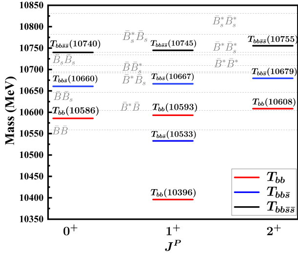
Fig. 2. (color online) Mass spectrum and spin-parity of doubly bottomed tetraquarks with nonstrange (red), single-strange (blue) and double-strange quarks (black).
