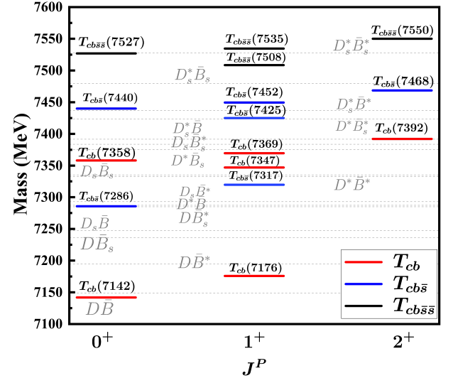
Fig. 3. (color online) Mass spectrum and spin-parity of bottom-charmed tetraquarks with nonstrange (red), single-strange (blue) and double-strange quarks (black).
