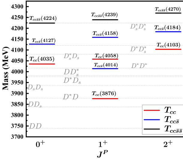
Fig. 1. (color online) Mass spectrum and spin-parity of doubly charmed tetraquarks with nonstrange (red), single-strange (blue) and double-strange quarks (black).
