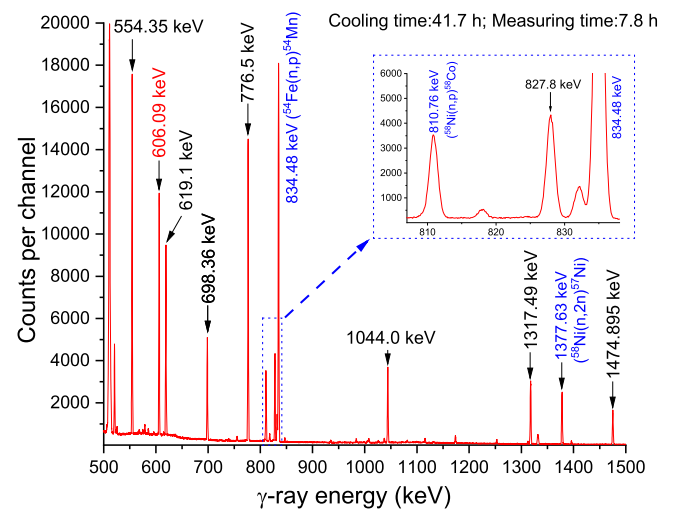
Fig. 5. (color online) The gamma spectrum of the krypton gas sample was measured after 2 hours of continuous neutron irradiation, followed by 41.7 hours of cooling, and the measurement time was 7.8 hours.
