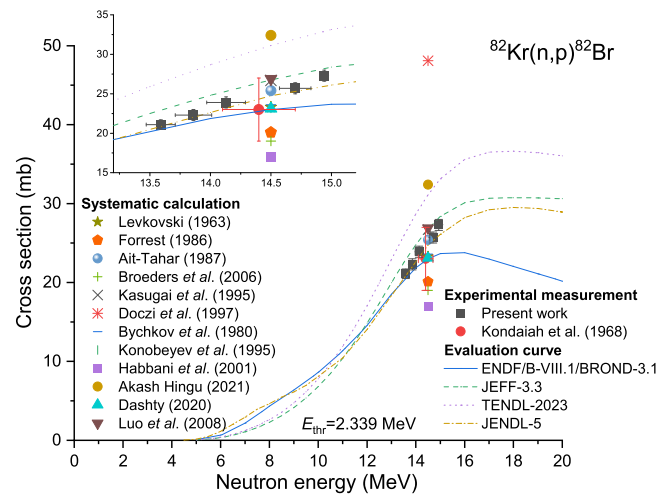
Fig. 7. (color online) Experimental data, systematic results, and evaluated curves for the ^{82}\text{Kr}(n, p)^{82}\text{Br} reaction.
