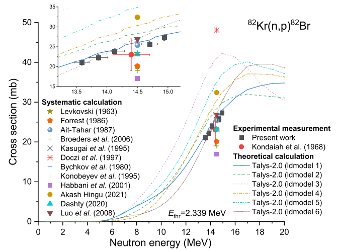
Fig. 6. (color online) Theoretical excitation function for the ^{82}\text{Kr}(n, p)^{82}\text{Br} reaction, along with experimental data and systematic results.
