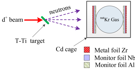
Fig. 3. (color online) Assembly diagram and relative position of sample group.
