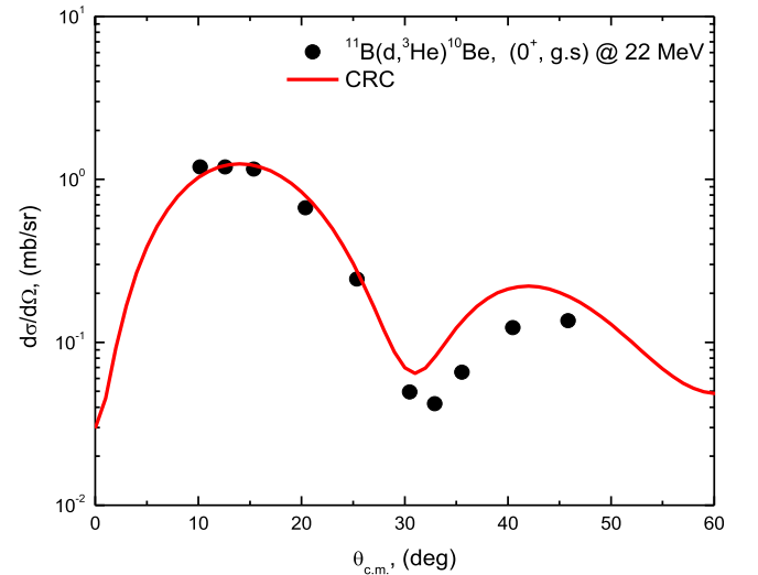
Fig. 6. (color online) Measured ADs for the {}^{11}\text{B}(d, {}^3\text{He}){}^{10}\text{Be} reaction at E_{\text{lab}} = 22 MeV, populating the ( 0^+ , 0.0 MeV) {}^{10}\text{Be} ground state (circles), compared with CRC calculations (curves)
