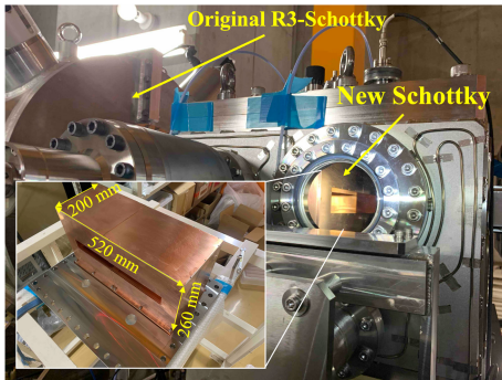
Fig. 4. (color online) New resonant Schottky pick-up, which has a rectangular shape, is installed in the existing vacuum chamber. The original pillbox-type R3-Schottky is located next to the new one.
