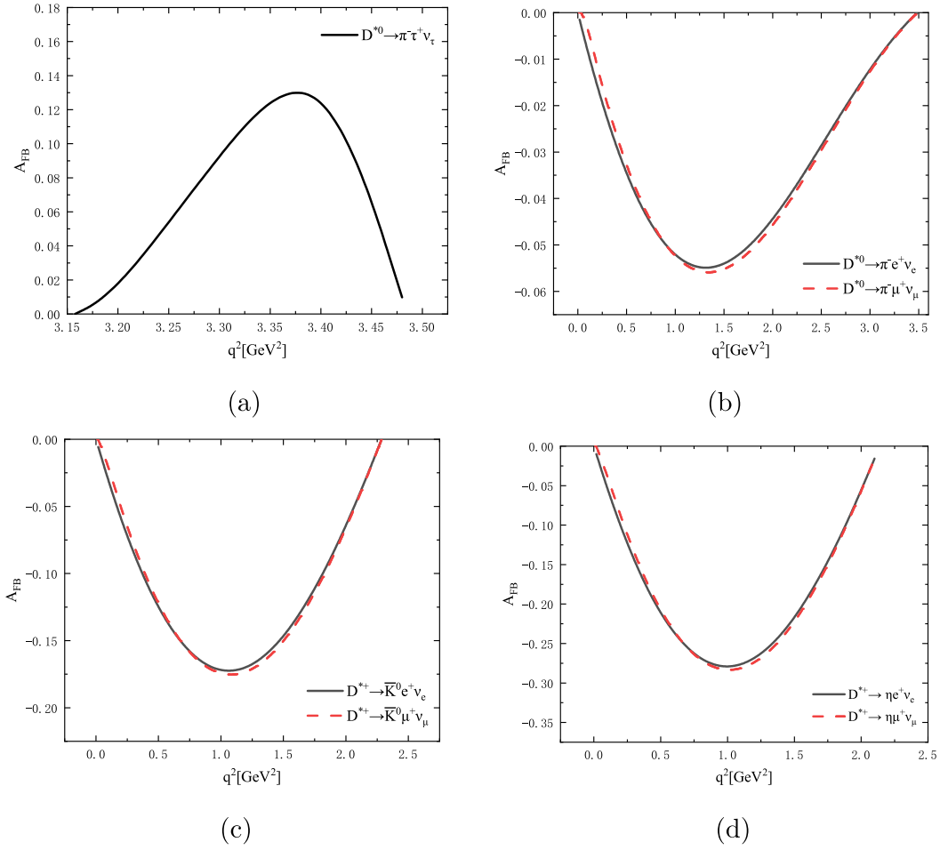
Fig. 3. (color online) q^2 -dependences of the forward-backward asymmetries A_{\text{FB}} for the decays D^{*0} \rightarrow \pi^- \tau^+ \nu_\tau (a), D^{*0} \rightarrow \pi^- \ell^+ \nu_\ell (b), D^{*+} \rightarrow \bar{K}^0 \ell^+ \nu_\ell (c), and D^{*+} \rightarrow \eta \ell^+ \nu_\ell (d).
