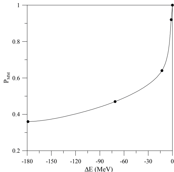
Fig. 1. P_{MM} as a function of \Delta E .
