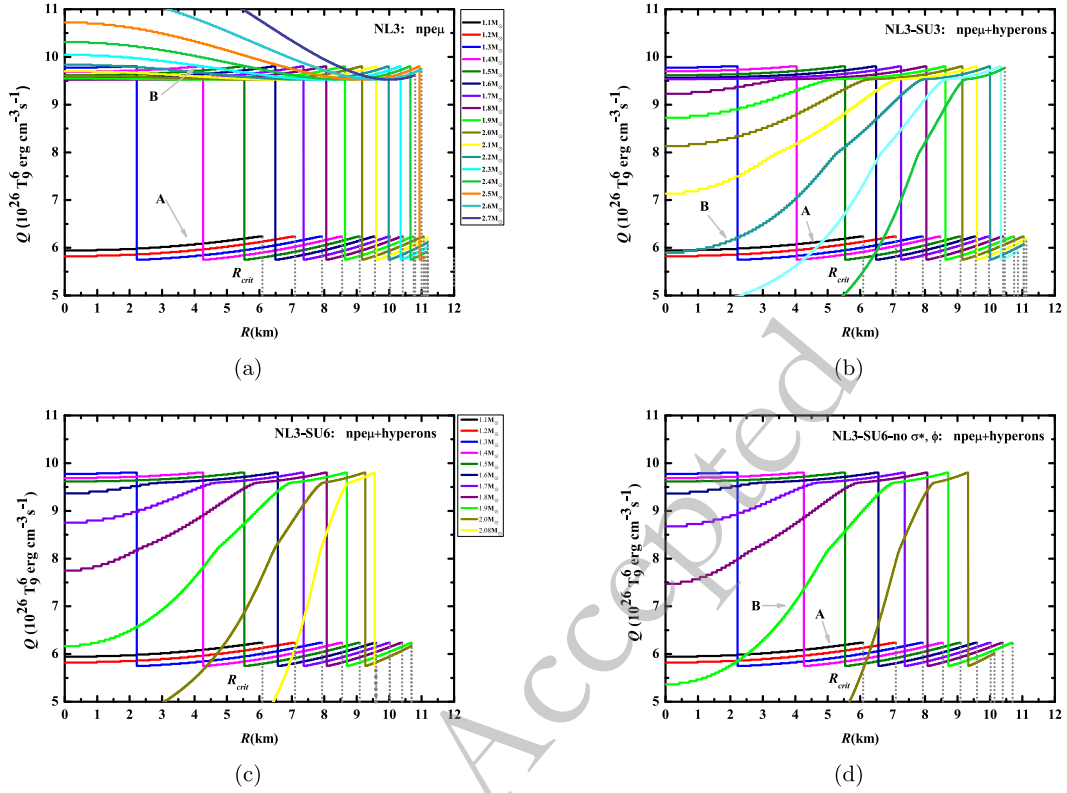
Fig. 3. (color online) Radial variation diagrams of the neutrino emissivity in the nucleonic direct Urca processes within the core of neutron stars are shown for four cases of the NL3 parameter set. The gray dotted lines represent the critical radius values at which the nucleonic direct Urca processes cease in neutron stars with different masses, respectively.
