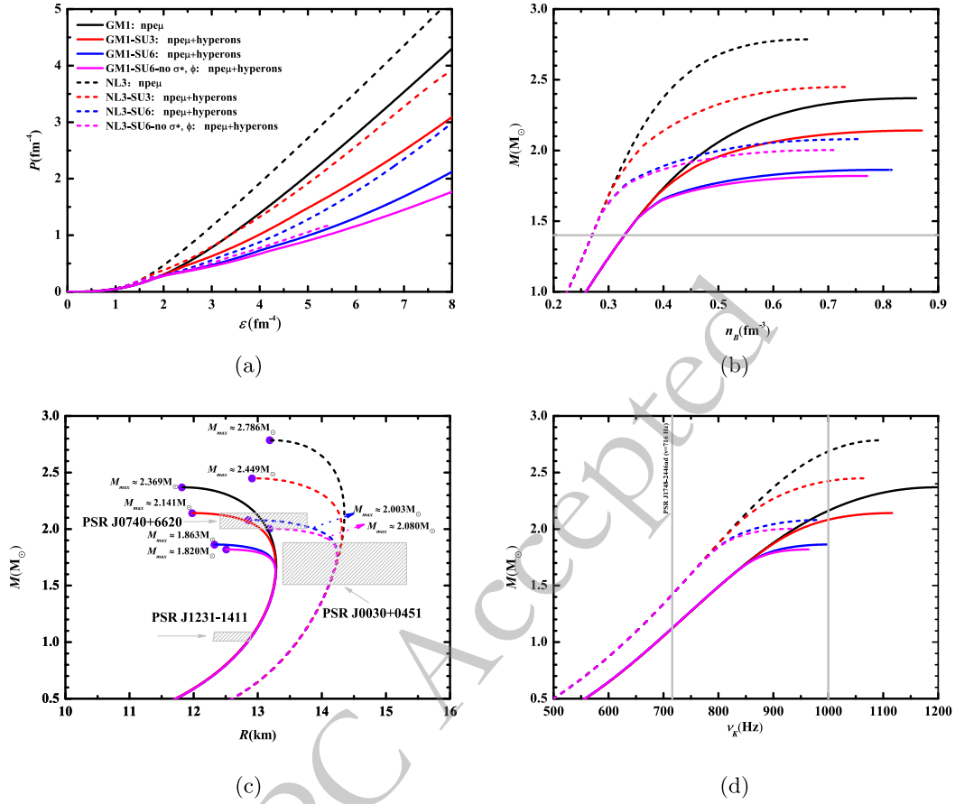
Fig. 1. (color online) The equations of state, mass-density, mass-radius, and mass-frequency relations of neutron stars are presented for four cases using the GM1 and NL3 parameter sets. The purple dots in Figure 1c represent the maximum mass values of neutron stars in each case.
