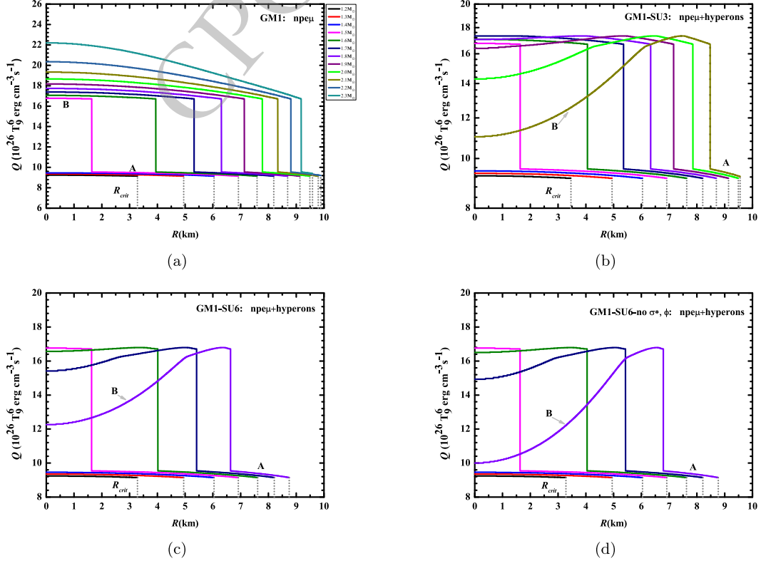
Fig. 2. (color online) Radial variation diagrams of the neutrino emissivity in the nucleonic direct Urca processes within the core of neutron stars are presented for four cases of the GM1 parameter set. The gray dotted lines represent the critical radius values at which the nucleonic direct Urca processes cease in neutron stars with different masses.
