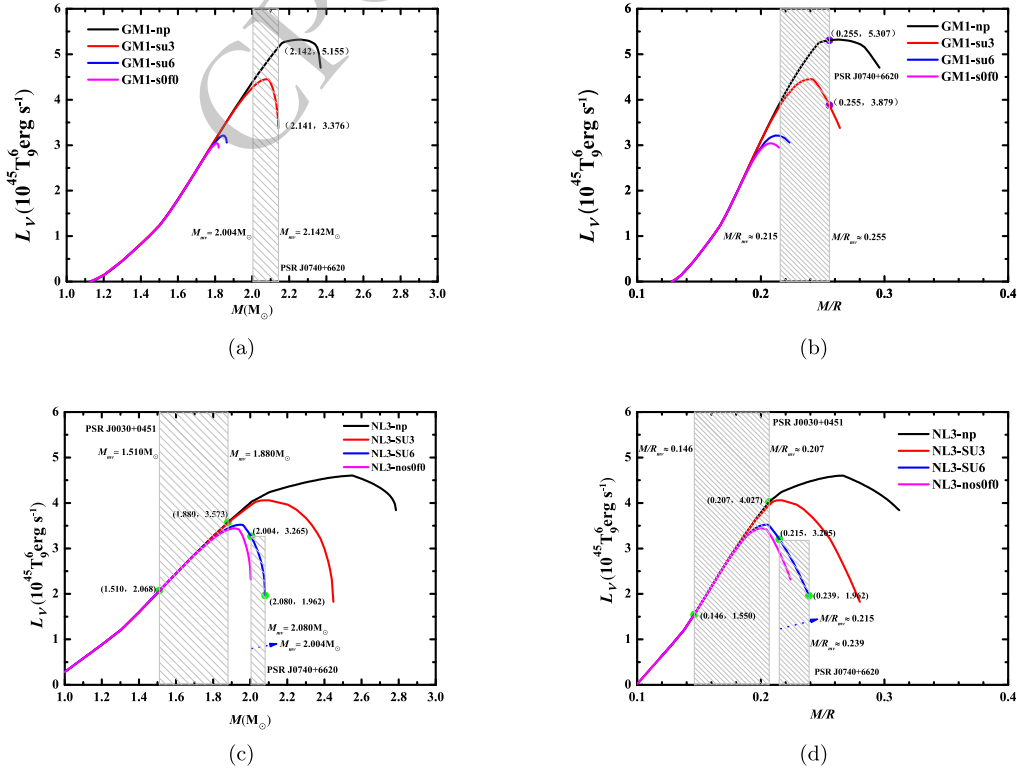
Fig. 4. (color online) Neutrino luminosity-mass and neutrino luminosity-compactness relations for four cases of the GM1 and NL3 sets are presented. Purple and green circles denote the theoretical prediction ranges of the neutrino luminosities for the nucleonic direct Urca processes in PSRs J0030+0451 and J0740+6620.
