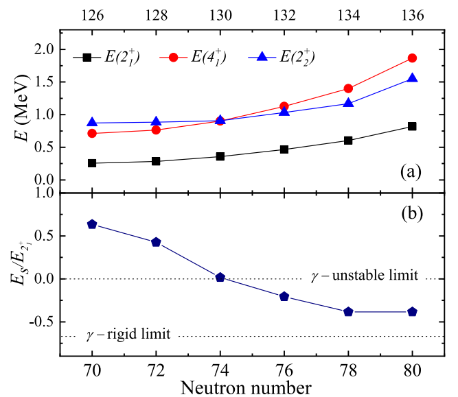
Fig. 1. (color online) (a) Energies of the first excited 2_1^+ , 4_1^+ , and 2_2^+ states, (b) energy ratio E_s/E_{2_1^+} .
