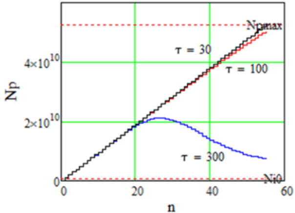
Fig. 13. (color online) Relationship between the number of stored ions ( N_p ) and injection cycles ( n ) for different cooling time constants ( \tau ).
