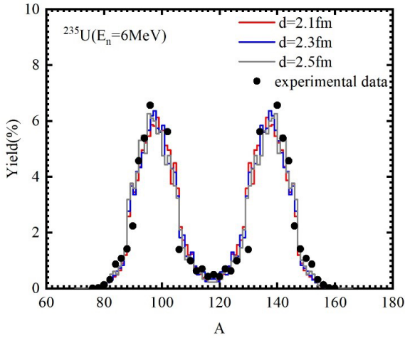
Fig. 3. (color online) Mass distributions of neutron-induced ^{235}\text{U} fission for different values of distance parameter d between two fragments.
