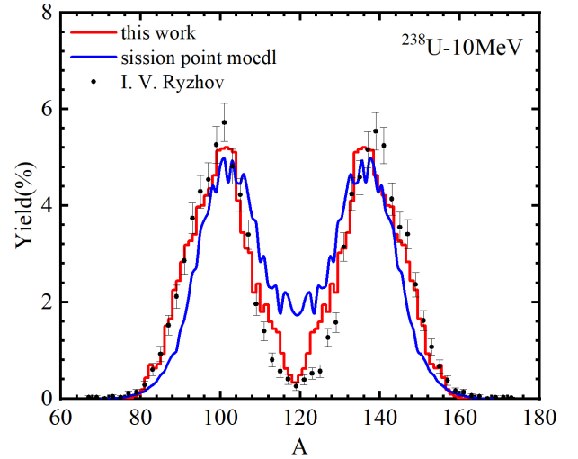
Fig. 11. (color online) Fission fragment mass distributions in neutron-induced ^{238}\text{U} fission and comparison with experimental data [28].
