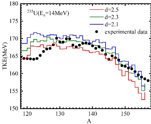
Fig. 4. (color online) Average total kinetic energy distributions of fragments of neutron-induced ^{235}\text{U} fission for different values of distance parameter d between two fragments and comparison with experimental data [22].
