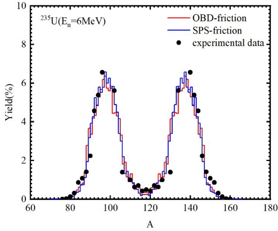
Fig. 5. (color online) Mass distributions of neutron-induced ^{235}\text{U} fission for different methods of the friction model.
