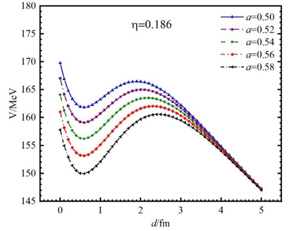
Fig. 6. (color online) Interaction potential energy of asymmetric fission.
