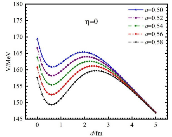
Fig. 7. (color online) Interaction potential energy of symmetric fission.
