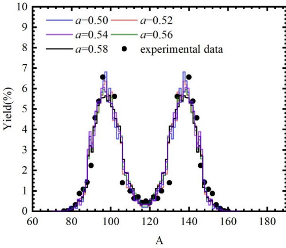
Fig. 9. (color online) Mass distribution for different diffuseness width parameters.
