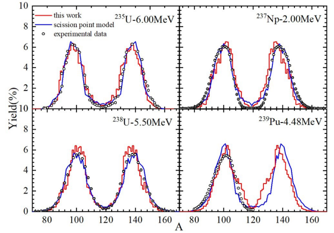
Fig. 10. (color online) Fission fragment mass distributions in neutron-induced ^{235,238}\text{U} , ^{237}\text{Np} and ^{239}\text{Pu} fission and comparison with the experimental data [24–27].
