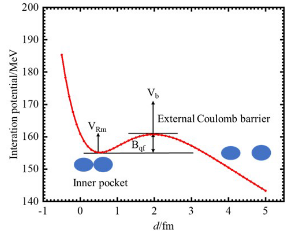
Fig. 2. (color online) Interaction potential energy of ^{96}\text{Sr} and ^{140}\text{Xe} in the reaction of n + ^{235}\text{U} .
