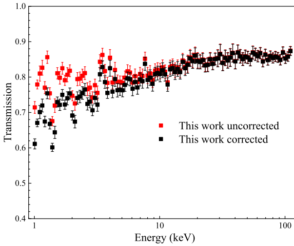
Fig. 11. (color online) Comparison of corrected (black) and uncorrected (red) transmissions from this study.
