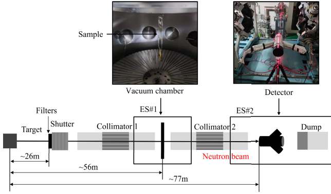
Fig. 2. (color online) Schematic diagram of neutron total cross section measurement facility. The sample was set at a vacuum chamber equipped with a remotely controlled sample-changing system. A wing-shaped lithium glass detector was employed at ES#2.
