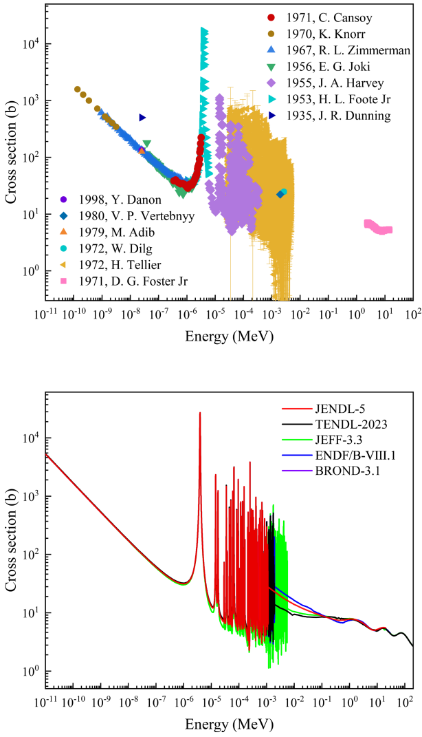
Fig. 1. (color online) Experimental cross section of ^{169}\text{Tm} from the EXFOR database (top panel) and evaluated cross section from ENDF/B-VIII.1, JENDL-5, JEFF-3.3, TENDL-2023, and BROND-3.1 libraries (bottom panel).
