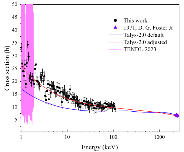
Fig. 13. (color online) Experimental data in the 1–110 keV range (black) compared with TALYS-2.0 calculations using default (blue) and adjusted (red) parameters and with evaluated data from TENDL-2023 (pink). When extended to 2.5 MeV, the adjusted parameters yield cross sections consistent with the results of Foster Jr. [34] in the 2.3–2.5 MeV range, with deviations mostly below 5%.
