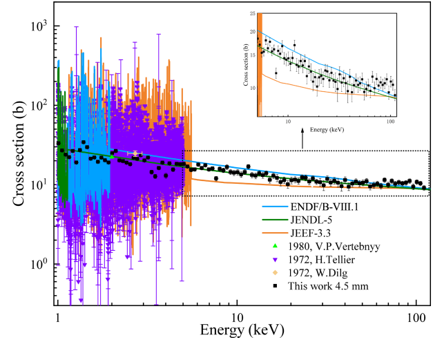
Fig. 12. (color online) Neutron total cross section measured in this study compared with ENDF/B-VIII.1 (blue), JENDL-5 (green), and JEFF-3.3 (orange) evaluations and EXFOR data.
