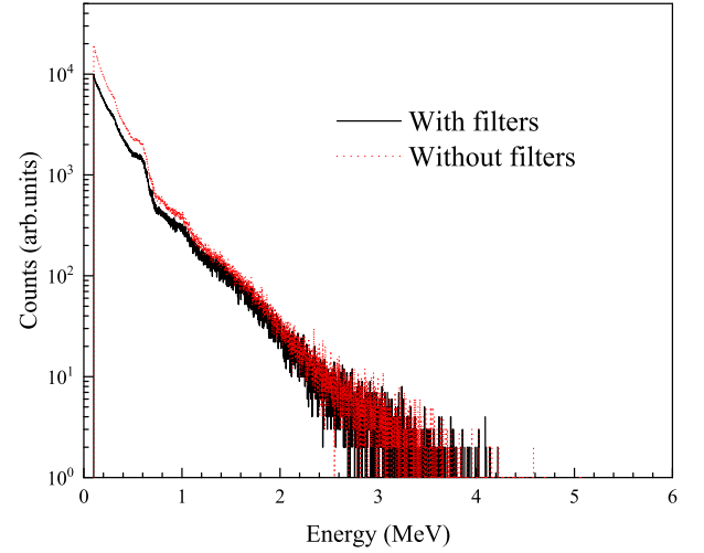
Fig. 9. (color online) Simulated spectra of the in-beam \gamma -ray energy for the ^7\text{Li} -GS detector. The solid line represents the values with filters, while the short-dashed line represents those without filters.
