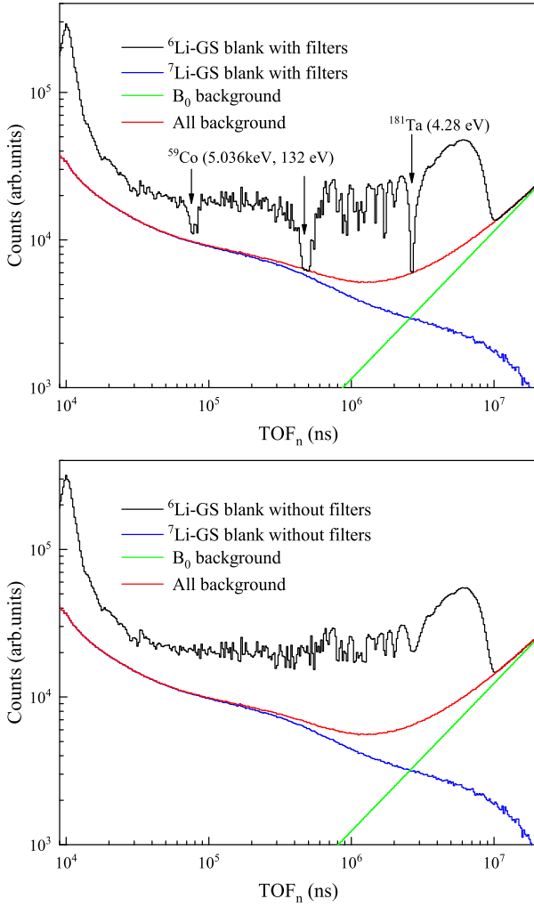
Fig. 8. (color online) Background composition without a sample measured by the ^6\text{Li} -GS and ^7\text{Li} -GS detectors. Top panel: background composition with filters. Bottom panel: background composition without filters.
