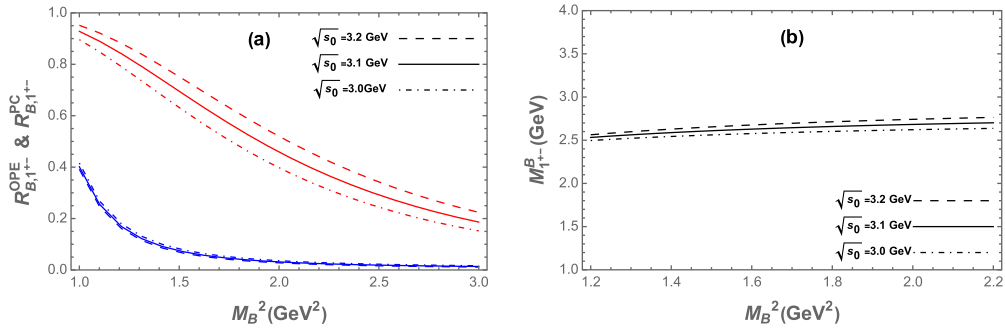
Fig. A11. (color online) (a) Ratios R_{B,1+-}^{OPE} and R_{B,1+-}^{PC} as functions of the Borel parameter M_B^2 for different values of \sqrt{s_0} for current (12), where blue lines represent R_{B,1+-}^{OPE} and red lines denote R_{B,1+-}^{PC} . (b) Mass of 1^{+-} fully strange tetraquark state as a function of the Borel parameter M_B^2 for different values of \sqrt{s_0} .
