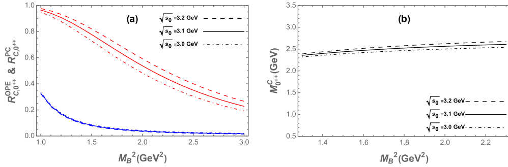
Fig. A2. (color online) (a) Ratios R_{C,0^{++}}^{\text{OPE}} and R_{C,0^{++}}^{\text{PC}} as functions of the Borel parameter M_B^2 for different values of \sqrt{s_0} for current (3), where blue lines represent R_{C,0^{++}}^{\text{OPE}} and red lines denote R_{C,0^{++}}^{\text{PC}} . (b) Mass of 0^{++} fully strange tetraquark state as a function of the Borel parameter M_B^2 for different values of \sqrt{s_0} .
