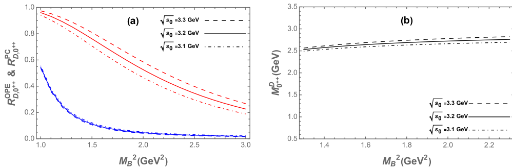
Fig. A3. (color online) (a) Ratios R_{D,0^{++}}^{\text{OPE}} and R_{D,0^{++}}^{\text{PC}} as functions of the Borel parameter M_B^2 for different values of \sqrt{s_0} for current (4), where blue lines represent R_{D,0^{++}}^{\text{OPE}} and red lines denote R_{D,0^{++}}^{\text{PC}} . (b) Mass of 0^{++} fully strange tetraquark state as a function of the Borel parameter M_B^2 for different values of \sqrt{s_0} .
