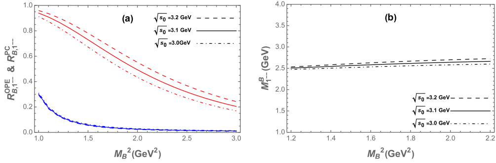
Fig. A9. (color online) (a) Ratios R_{B,1--}^{OPE} and R_{B,1--}^{PC} as functions of the Borel parameter M_B^2 for different values of \sqrt{s_0} for current (10), where blue lines represent R_{B,1--}^{OPE} and red lines denote R_{B,1--}^{PC} . (b) Mass of 1^{--} fully strange tetraquark state as a function of the Borel parameter M_B^2 for different values of \sqrt{s_0} .
