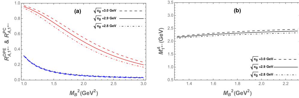
Fig. A10. (color online) (a) Ratios R_{A,1+-}^{OPE} and R_{A,1+-}^{PC} as functions of the Borel parameter M_B^2 for different values of \sqrt{s_0} for current (11), where blue lines represent R_{A,1+-}^{OPE} and red lines denote R_{A,1+-}^{PC} . (b) Mass of 1^{+-} fully strange tetraquark state as a function of the Borel parameter M_B^2 for different values of \sqrt{s_0} .
