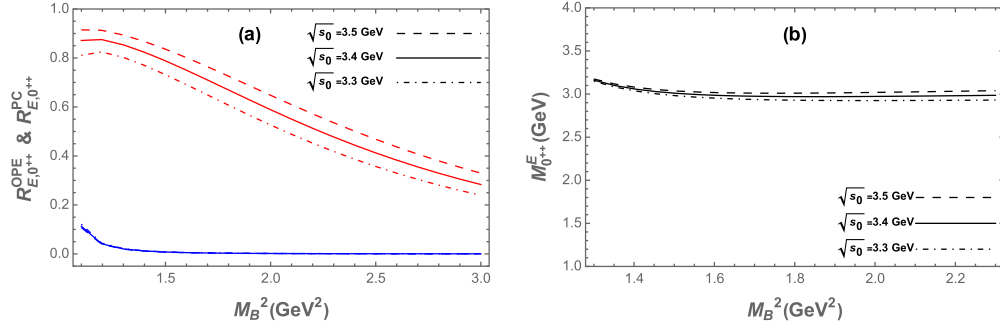
Fig. A4. (color online) (a) Ratios R_{E,0^{++}}^{OPE} and R_{E,0^{++}}^{PC} as functions of the Borel parameter M_B^2 for different values of \sqrt{s_0} for current (5), where blue lines represent R_{E,0^{++}}^{OPE} and red lines denote R_{E,0^{++}}^{PC} . (b) Mass of 0^{++} fully strange tetraquark state as a function of the Borel parameter M_B^2 for different values of \sqrt{s_0} .
