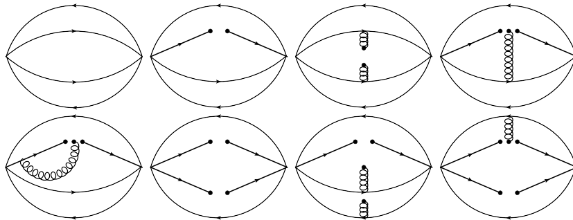
Fig. 1. Typical Feynman diagrams related to the correlation function, where the solid lines denote quarks and spiral ones denote gluons.
