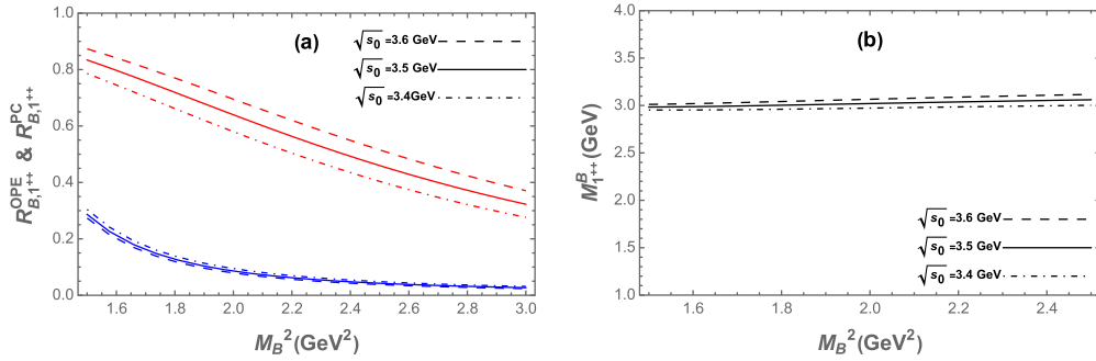
Fig. A13. (color online) (a) Ratios R_{B,1^{++}}^{OPE} and R_{B,1^{++}}^{PC} as functions of the Borel parameter M_B^2 for different values of \sqrt{s_0} for current (14), where blue lines represent R_{B,1^{++}}^{OPE} and red lines denote R_{B,1^{++}}^{PC} . (b) Mass of 1^{++} fully strange tetraquark state as a function of the Borel parameter M_B^2 for different values of \sqrt{s_0} .
