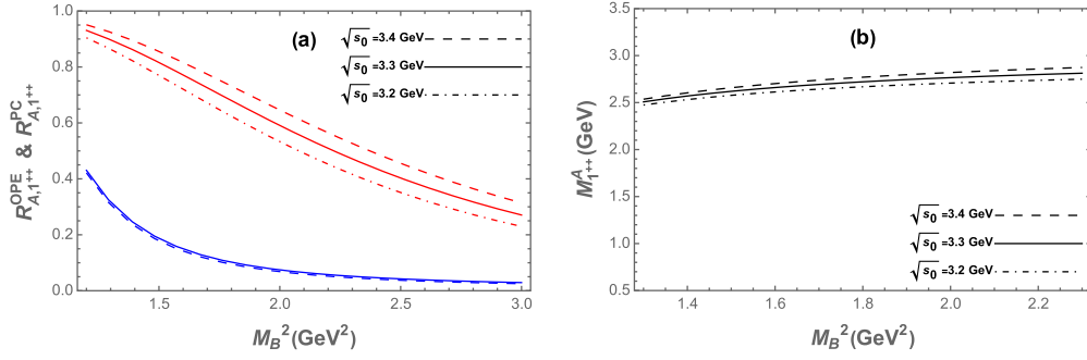
Fig. A12. (color online) (a) Ratios R_{A,1^{++}}^{OPE} and R_{A,1^{++}}^{PC} as functions of the Borel parameter M_B^2 for different values of \sqrt{s_0} for current (13), where blue lines represent R_{A,1^{++}}^{OPE} and red lines denote R_{A,1^{++}}^{PC} . (b) Mass of 1^{++} fully strange tetraquark state as a function of the Borel parameter M_B^2 for different values of \sqrt{s_0} .
