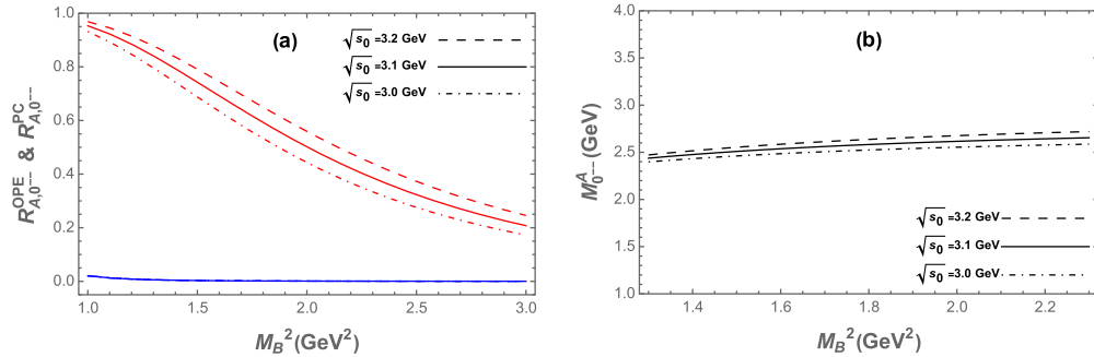
Fig. A7. (color online) (a) Ratios R_{A,0^{--}}^{OPE} and R_{A,0^{--}}^{PC} as functions of the Borel parameter M_B^2 for different values of \sqrt{s_0} for current (8), where blue lines represent R_{A,0^{--}}^{OPE} and red lines denote R_{A,0^{--}}^{PC} . (b) Mass of 0^{--} fully strange tetraquark state as a function of the Borel parameter M_B^2 for different values of \sqrt{s_0} .
