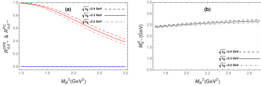
Fig. A5. (color online) (a) Ratios R_{A,0^{+-}}^{OPE} and R_{A,0^{+-}}^{PC} as functions of the Borel parameter M_B^2 for different values of \sqrt{s_0} for current (6), where blue lines represent R_{A,0^{+-}}^{OPE} and red lines denote R_{A,0^{+-}}^{PC} . (b) Mass of 0^{+-} fully strange tetraquark state as a function of the Borel parameter M_B^2 for different values of \sqrt{s_0} .
