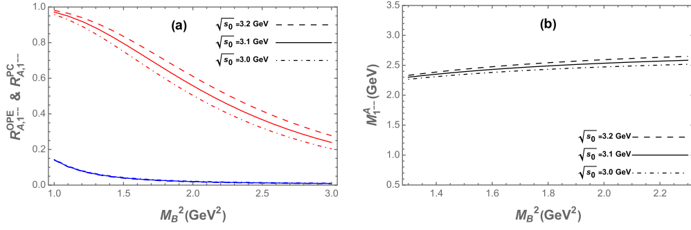
Fig. A8. (color online) (a) Ratios R_{A,1--}^{OPE} and R_{A,1--}^{PC} as functions of the Borel parameter M_B^2 for different values of \sqrt{s_0} for current (9), where blue lines represent R_{A,1--}^{OPE} and red lines denote R_{A,1--}^{PC} . (b) Mass of 1^{--} fully strange tetraquark state as a function of the Borel parameter M_B^2 for different values of \sqrt{s_0} .
