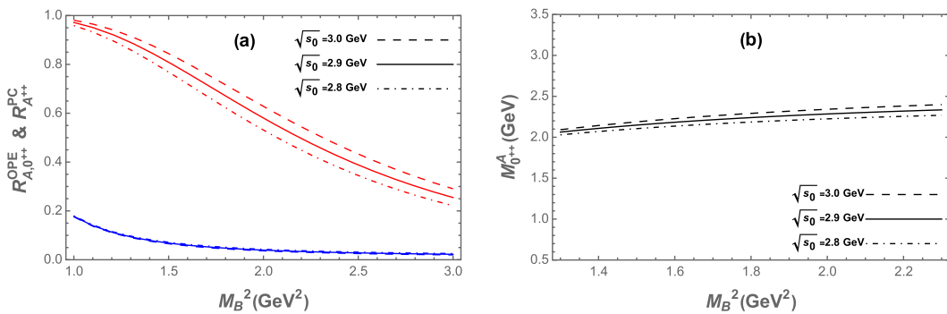
Fig. 2. (color online) (a) Ratios R_{A,0^{++}}^{\text{OPE}} and R_{A,0^{++}}^{\text{PC}} as functions of the Borel parameter M_B^2 for different values of \sqrt{s_0} for current (1), where blue lines represent R_{A,0^{++}}^{\text{OPE}} and red lines denote R_{A,0^{++}}^{\text{PC}} . (b) Mass of 0^{++} fully strange tetraquark state as a function of the Borel parameter M_B^2 for different values of \sqrt{s_0} .
