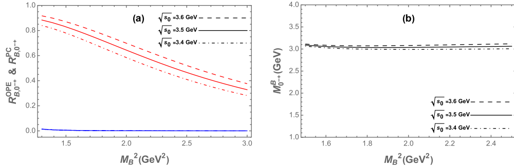
Fig. A6. (color online) (a) Ratios R_{B,0^{++}}^{OPE} and R_{B,0^{++}}^{PC} as functions of the Borel parameter M_B^2 for different values of \sqrt{s_0} for current (7), where blue lines represent R_{B,0^{++}}^{OPE} and red lines denote R_{B,0^{++}}^{PC} . (b) Mass of 0^{++} fully strange tetraquark state as a function of the Borel parameter M_B^2 for different values of \sqrt{s_0} .
