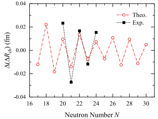
Fig. 3. (color online) Evolution of \Delta(\Delta R_{\text{ch}}) derived from Eq. (5) according to neutron numbers. Experimental data are taken from Refs. [14, 15, 26, 82].
