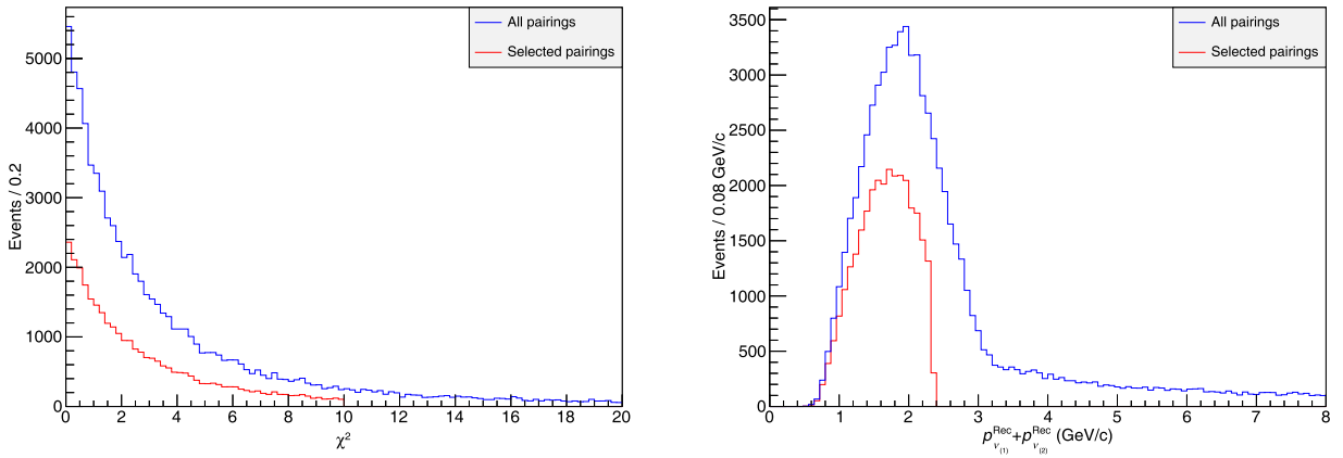
Fig. 6. (color online) Distribution of \chi^2 (left panel) and p_\nu = p_{\nu(1)} + p_{\nu(2)} (right panel) for selected pairings and all pairings.
