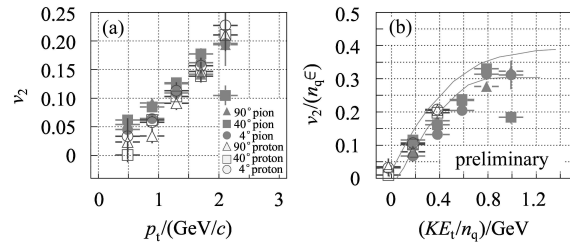
Fig. 3. (a) v_2(p_t) vs. p_t for pions and protons at \eta=0,1 , and 3 ; (b) Constituent quark scaled values, as discussed in the text. The lines indicate the band containing most of the previous experimental results near mid-rapidity.
