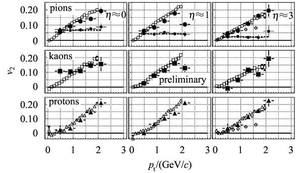
Fig. 1. v_2(p_t, \eta) for pions (both charges), kaons (both charges), and protons (filled symbols). Theoretical values based on the hydrodynamic calculations of Hirano et al. [7] are shown by the open circles, squares, and triangles. The open crosses correspond to \eta \approx 4 calculations using the AMPT model [8] . The smaller (blue in color) points in the pion panels are from a mixed-event analysis, as discussed in the text.
