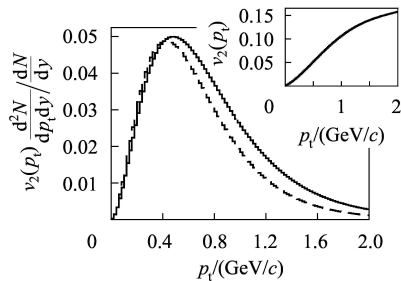
Fig. 2. Illustration of how the softening of the particle spectra going to forward angles affects the integral v_2 values. The insert shows the general behavior of the differential v_2(p_t) values for pions, which for this illustration is assumed to be independent of pseudorapidity. Folding this distribution with the corresponding experimentally observed pion spectra at 4^\circ and 90^\circ results in the dashed and solid curves, with integral v_2 values of 0.046 and 0.036, respectively.
