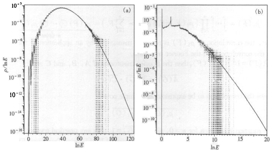
Fig. 1. The experiment estimator probability density functions for a Gaussian event estimator probability function (a) and for a typical non-Gaussian event estimator (b).
